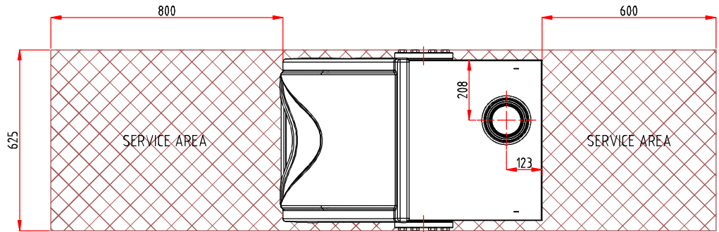
TOP VIEW
