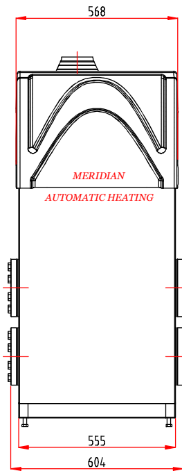
FRONT VIEW
