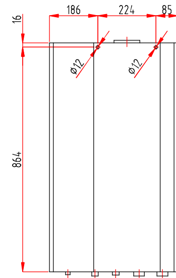
REAR VIEW
